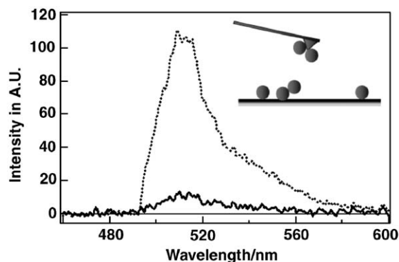
Fig. 2. Fluorescence spectra of GFP molecules measured when a large compression force of over 1 \mu N was applied. The solid line expresses the fluorescence spectrum in the contact area. It was acquired after applying the compression force to the measurement point of the CLSM and retracting the AFM probe completely from the substrate surface. The dotted line is the fluorescence spectrum of GFPs outside the contact area.
