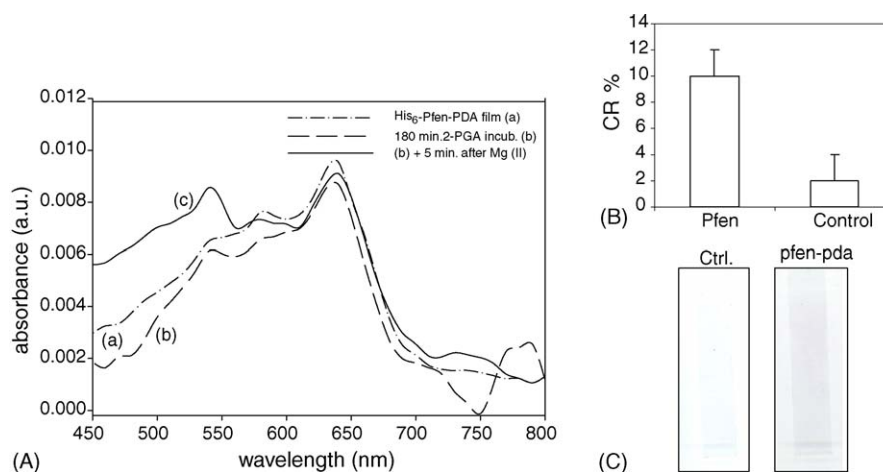
Fig. 7. UV-vis spectra of His 6 -Pfen-PDA film upon binding Mg (II) and 2-PGA. (A) (a) A His 6 -Pfen-PDA film in 50 mM Tris of pH = 7.6 (background); (b) at 180 min after the addition of 1.5 mM 2-PGA; (c) 1.5 mM Mg (II) added to the film in (b) and incubated for 5 min. (B) Plot of CR % vs. r-Pfen and control. (C) Colour change of a Pfen film with respect to a control film. A slight red tinge is observable with naked eyes for Pfen-PDA film.
