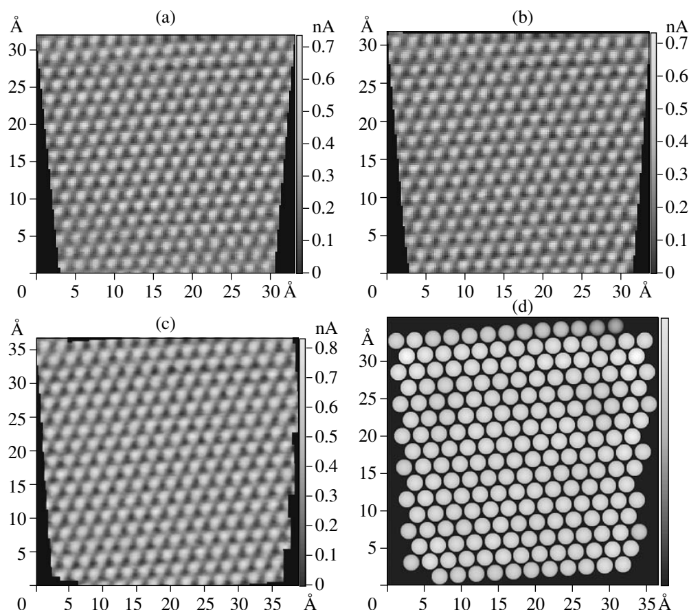
Fig. 2. Corrected atomic surface relief of pyrolytic graphite: (a) the linear correction, the average error over the image field is 0.3%; (b) the nonlinear correction performed using regression surfaces, the average error over the image field is 0.09%; and (c) the nonlinear correction using relief assembling from separate partially overlapping surface segments. The averaged lattice constant is 2.4638 Å, which corresponds to the relative measurement error of 0.01%. (d) The spherical model of the surface in panel (c).
